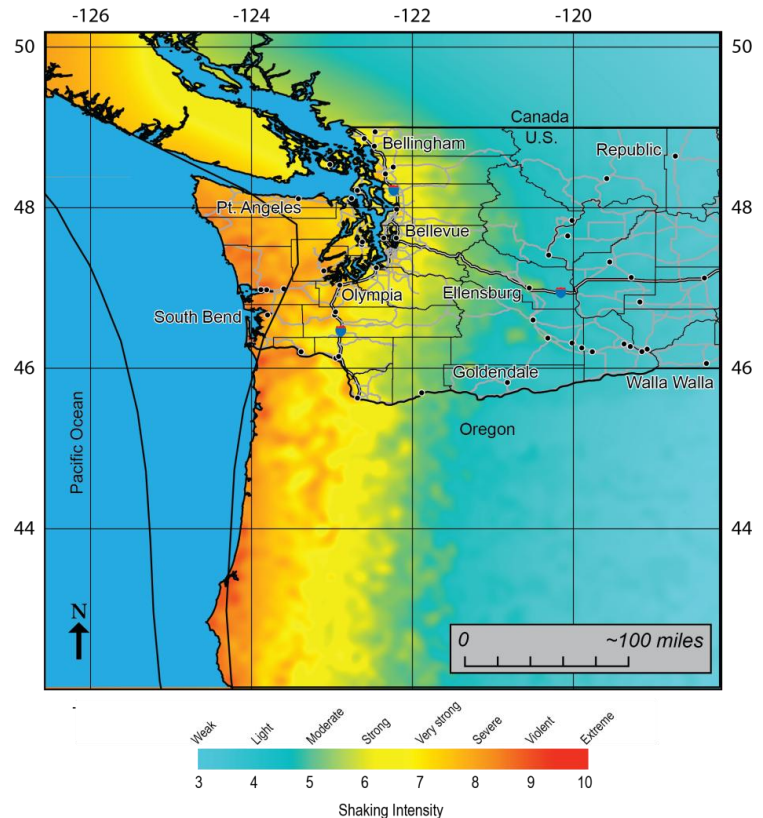
Figure 1. Earthquake planning scenario instrumental intensity map for a M9.0 earthquake on the Cascadia megathrust. The black polygon offshore is the modeled fault rupture for this scenario.
