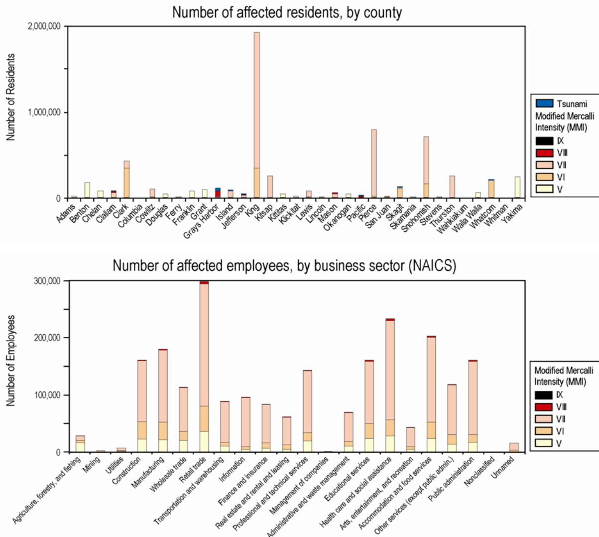
Figure 3. Number of residents and employees affected by the M9.0 earthquake projected for the Cascadia subduction zone. Modified Mercalli Intensity (MMI) classes indicate peak ground acceleration (PGA) values and the impact of the shaking.
